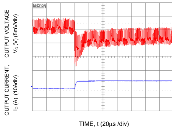
Figure 4. Transient Response to Dynamic Load Change from 50% to 100% at 12Vin, C_{out}=3 \times 47\mu F + 6 \times 330\mu F , C_{Tune}=47nF , R_{Tune}=180\Omega
