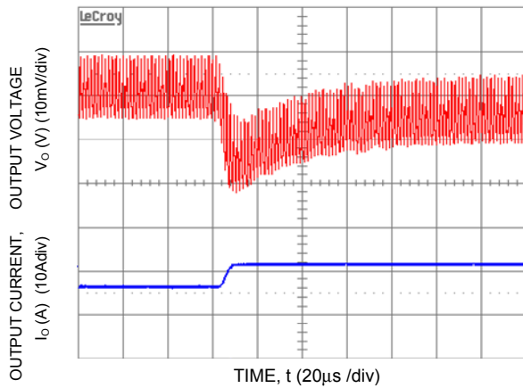
Figure 10. Transient Response to Dynamic Load Change from 50% to 100% at 12Vin, Cout-1x47μF+3x330uF, CTune-10nF & RTune-220ohms
