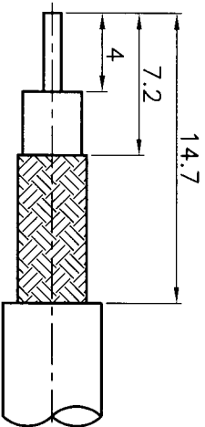
RECOMMENDED CABLE STRIPPING DIM'S
