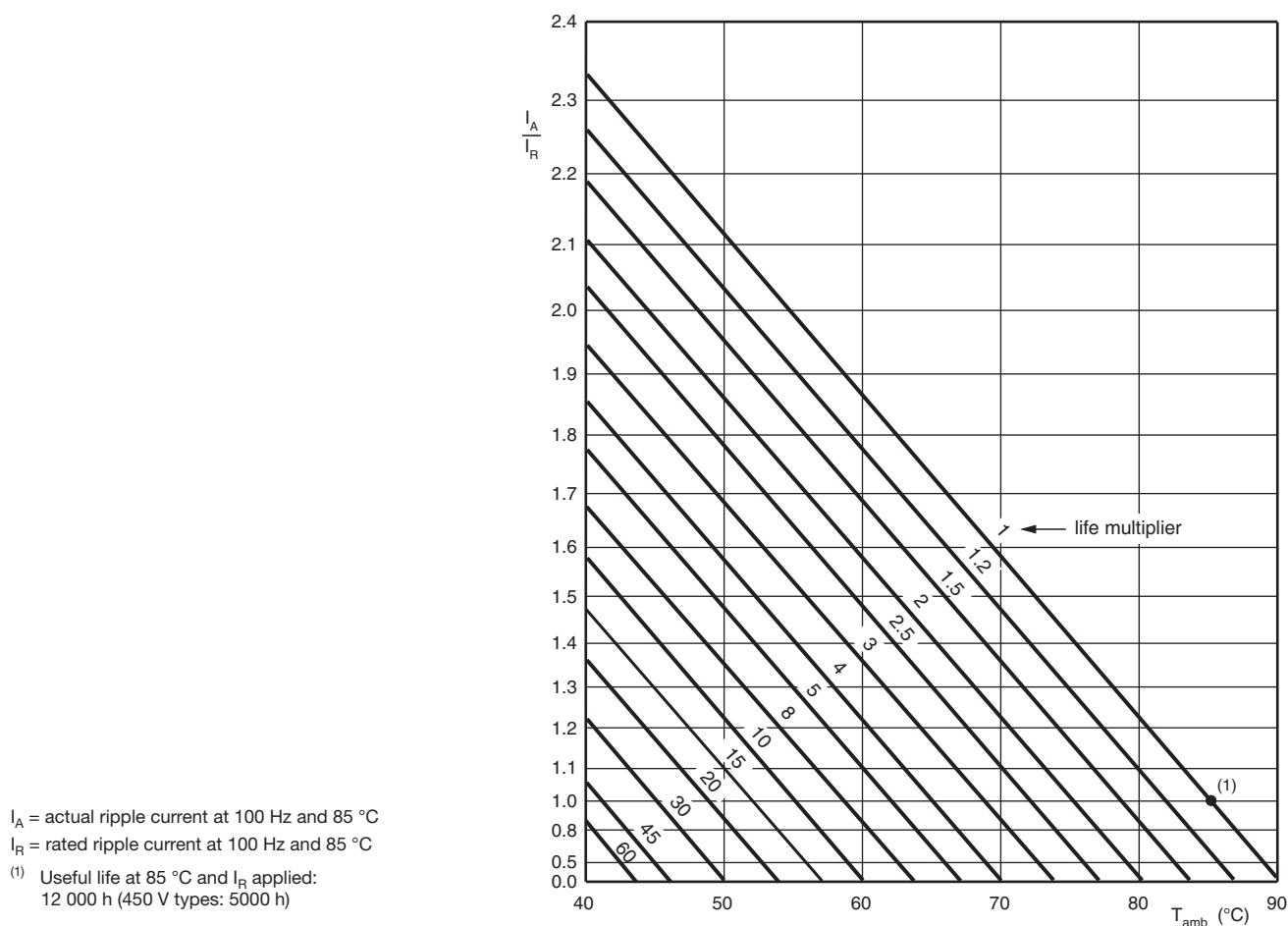
Fig. 18 - Multiplier of useful life as a function of ambient temperature and ripple current load
