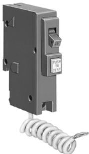
HOM 1-Pole GFI with ground fault circuit interrupter; 1 space required.
