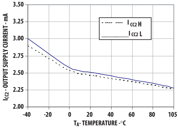
Figure 6. I_{CQ} vs. temperature
