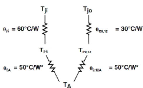
Figure 39. ACPL-330J Thermal Model
