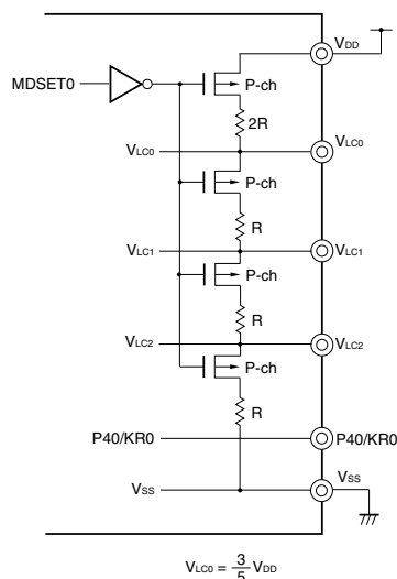
(b) 1/3 bias method and static display mode (MDSET1, MDSET0 = 1, 1) (example of V_{DD} = 5V , V_{LC0} = 3V )
