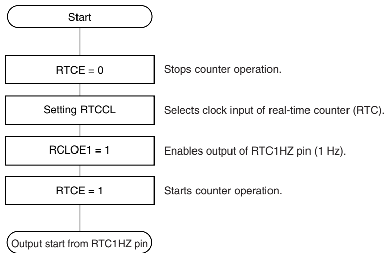
Figure 9-24. 1 Hz Output Setting Procedure
