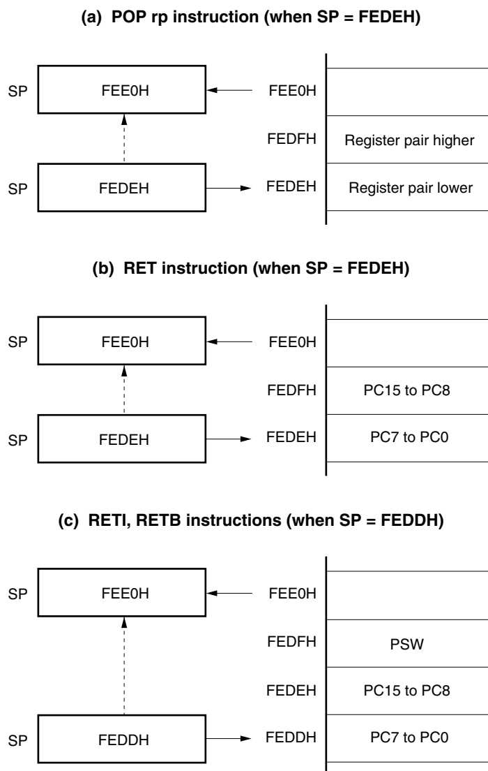
Figure 3-17. Data to Be Restored from Stack Memory
