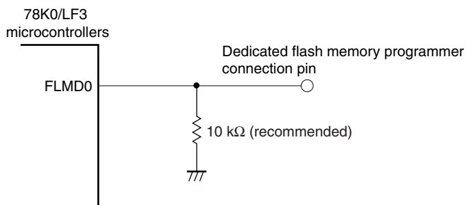
Figure 28-6. FLMD0 Pin Connection Example
