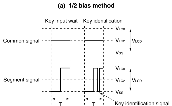
Figure 18-19 Voltages and Phases of Common and Segment Signals
