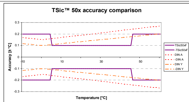
Figure 1: Comparison of TSic™ <--> platinum sensor
