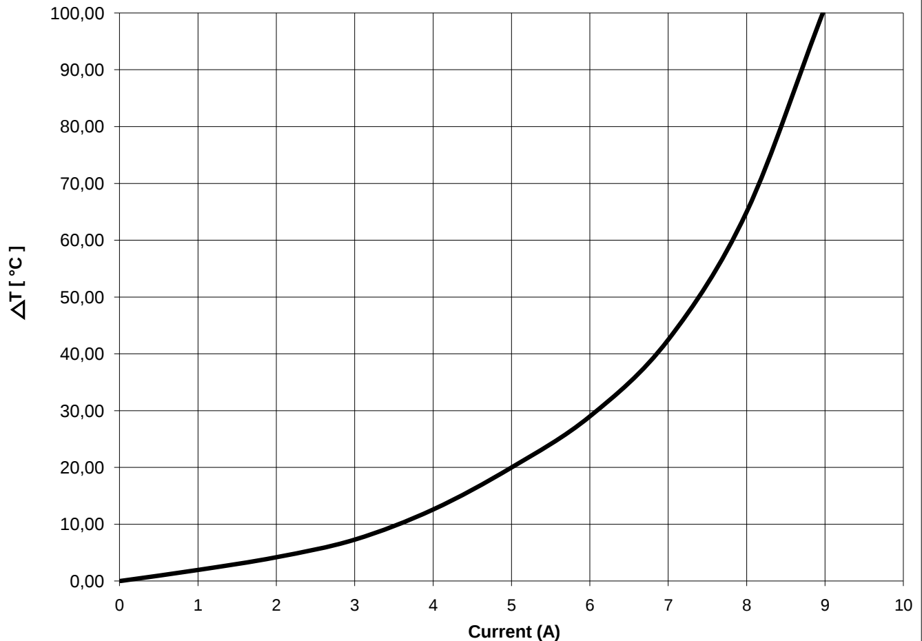
Temperaturanstieg vs. Strom (typ.)/ Temperature rise vs. Current (typ.)
