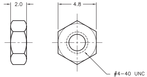
Nut (2 pcs)
