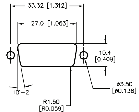
Panel Cutout
