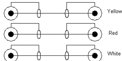
Wiring Diagram
