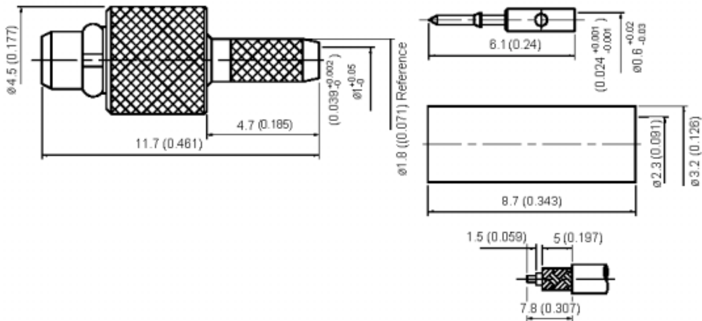
Stripping Dimension
