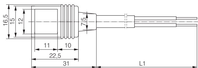
Connector cable Straight plug (G)
