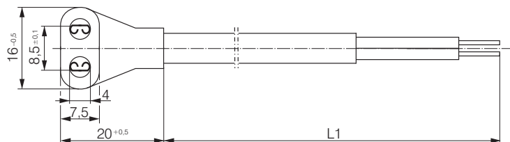
Connector cable Angled plug (W)
