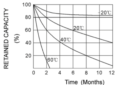
SELF DISCHARGE RATE AT VARIOUS TEMPERATURES
