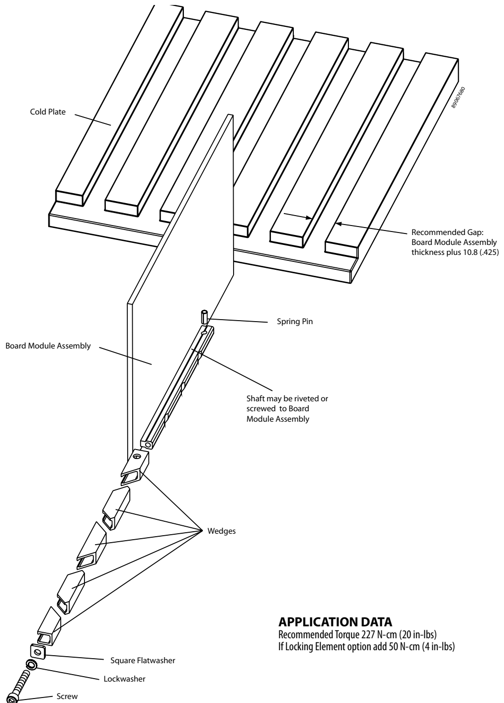
Series 280 - "Card-Lok" Retainer (Cold Plate)
