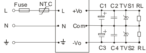
PH**-10A**(Dual Output)
