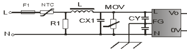
Figure 2. Input filter circuit
