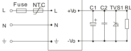
PH**-10D**(Isolate Twin Output)
