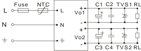
EXTERNAL CAPACITORS TYPICAL VALUE(Unit: mF)
