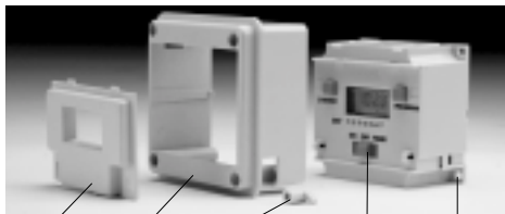
Tamper proof cover Bezel for panel mounting Panel mount bolts Slide switch allowing continuous ON or OFF or programmed operation Surface mount fixing
