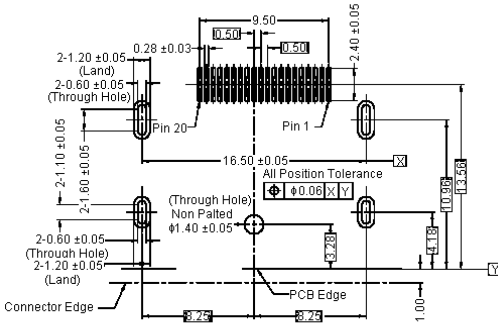
Recommend PCB Layout (Thickness = 1.6 ± 0.15mm)
