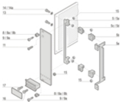
Item 9a, 3 U front panel mounting
