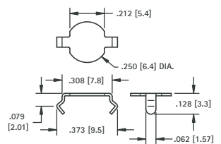
DWG. 2 MATERIAL: .010 (.25) Phosphor Bronze
