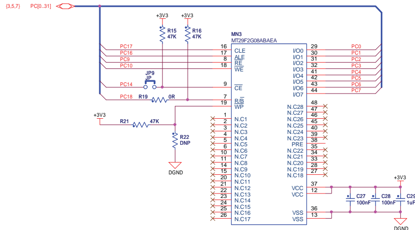
Figure 4-2. NAND Flash
