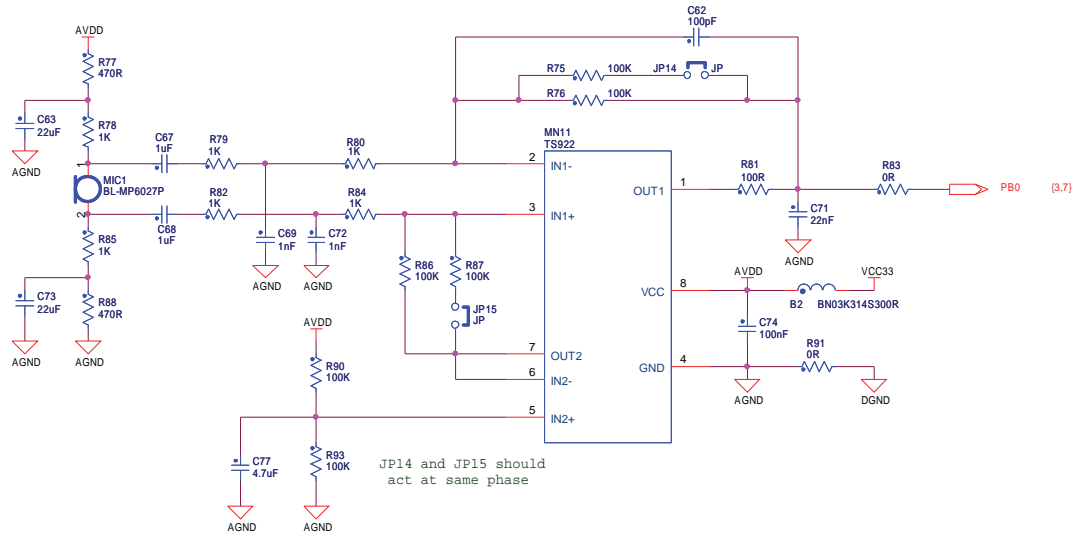
Figure 4-12. Microphone Input
