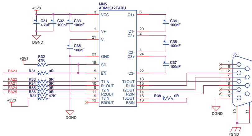
Figure 4-6. USART Evaluation Kit Hardware
