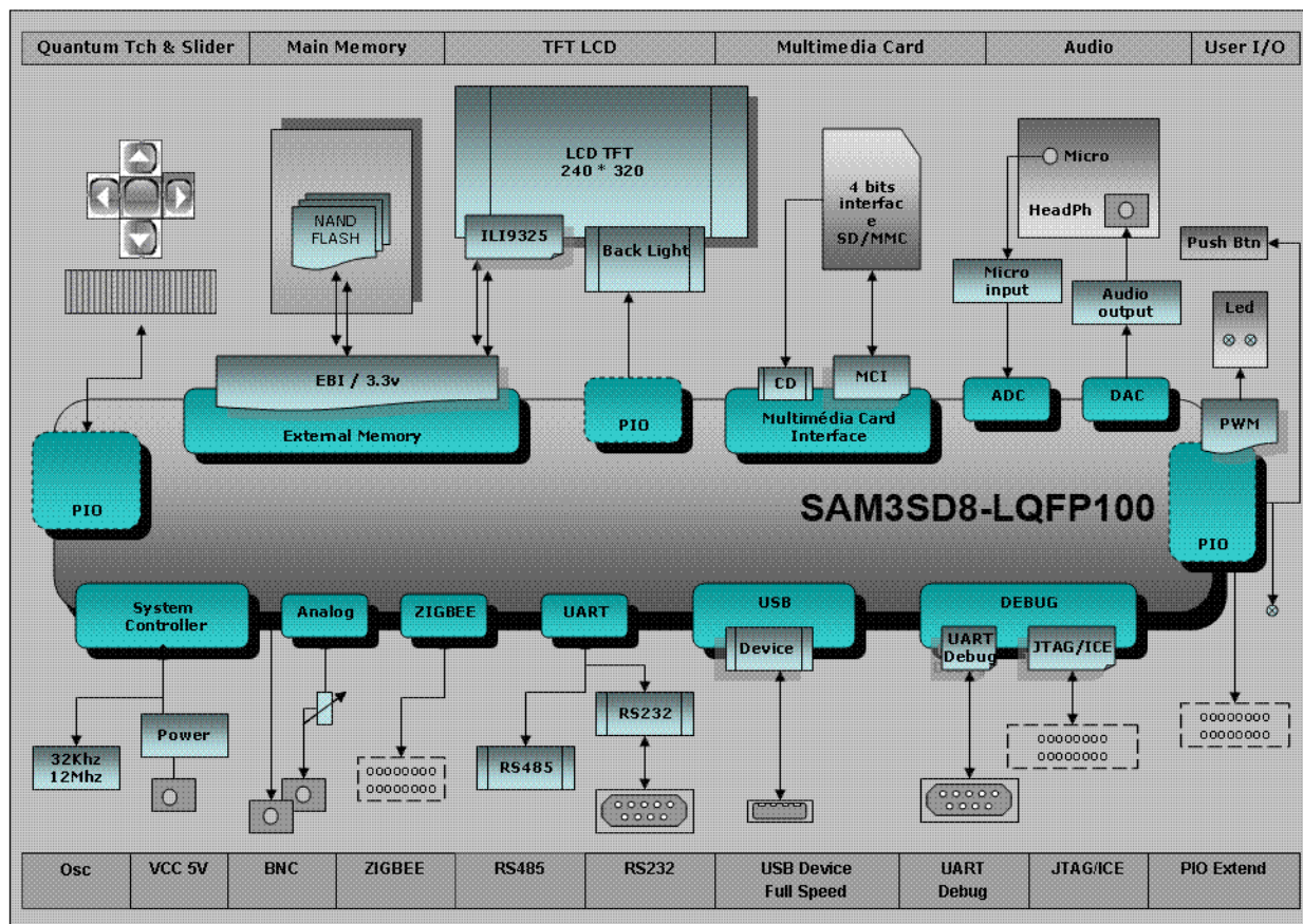
Figure 4-1. SAM3S-EK2 Block Diagram
