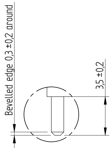
DETAIL A (5:1)
