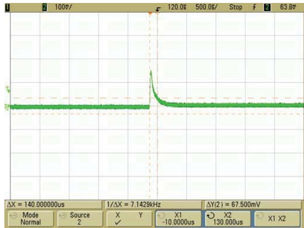
Step Load Transient Response (Slew=1A / \mu Sec., Vin=48V., Clad=0, Iout=15A to 22.5A)
