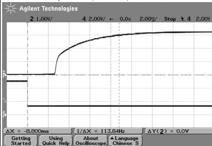
On/Off Enable Delay (Vin=48V, Vout=nom., Iout=30A, Clad=10uF, Ta=+25° C., ScopeBW=20Mhz, Trace 2=Vout, Trace 4=Enable).
