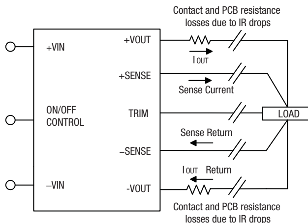
Figure 9. Remote Sense Circuit Configuration
