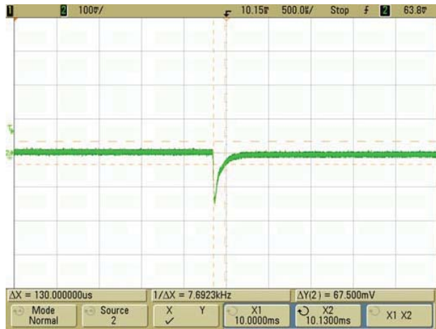
Step Load Transient Response (Slew=1A / \mu Sec., Vin=48V., Clad=0, Iout=22.5A to 15A)
