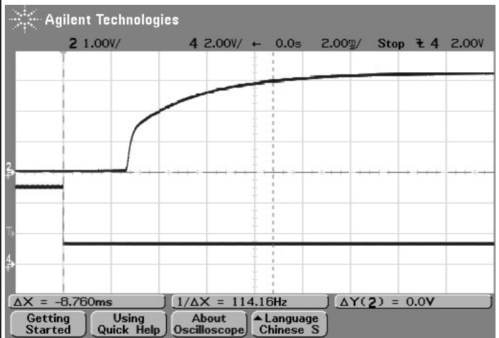
On/Off Enable Delay (Vin=48V, Vout=nom., Iout=25A, Clad=10uF, Ta=+25° C., ScopeBW=20Mhz, Trace 2=Vout, Trace 4=Enable.
