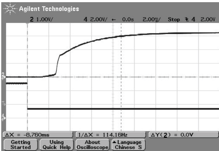
On/Off Enable Delay (Vin=48V, Vout=nom., Iout=0A, Clad=0, Ta=+25° C., ScopeBW=20Mhz, Trace 2=Vout, Trace 4=Enable.
