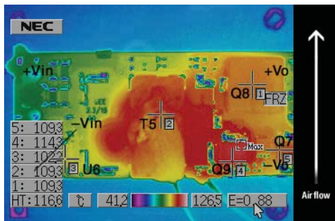
Thermal image with hot spot at full load current with 85 °C ambient; air is flowing at 100 LFM. Air is flowing across the converter from -Vin to +Vin at 48V input. Identifiable and recommended maximum value to be verified in application. Q9, Max temp= 120 °C/IPC9592 derating guidelines.
