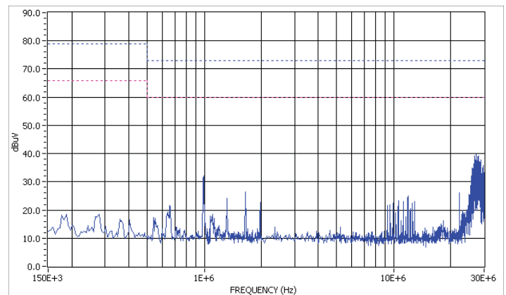
Graph 4. Conducted emissions performance, Negative Line, CISPR 22, Class A, full load
