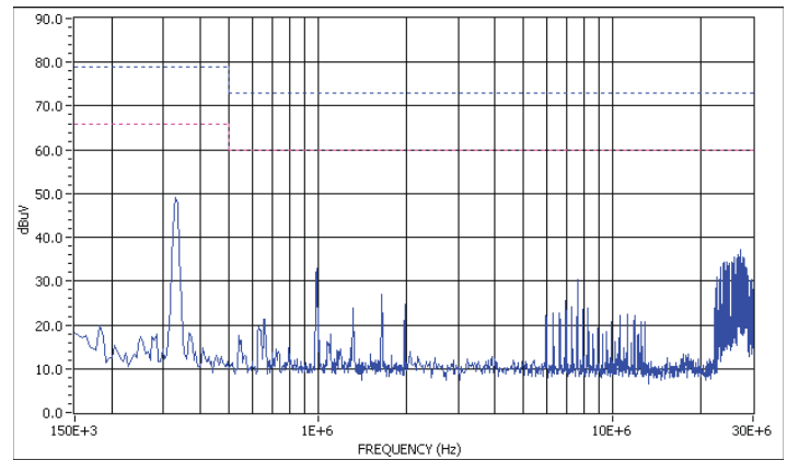
Graph 3. Conducted emissions performance, Positive Line, CISPR 22, Class A, full load
