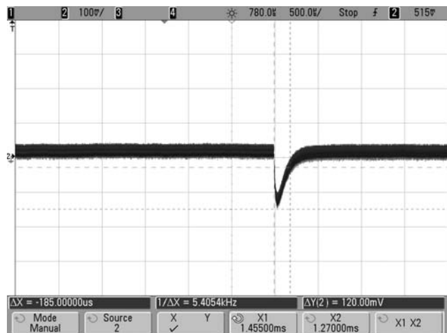
Step Load Transient Response (Vin=48V, Vout=nominal, Cload=0, Iout=50% to 75% of full load, Ta=+25°C.) Trace 1=Vout, 100 mV/div., 500 µS/div.
