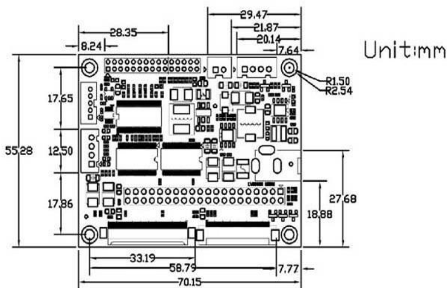
LVDS8000 Adapter Board Dimension Chart
