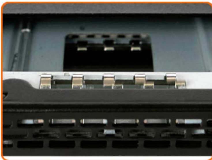
EMI GROUNDING + ANTI-VIBRATION DESIGN
