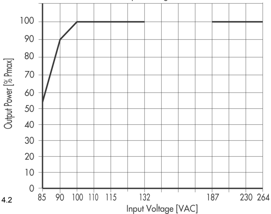
B) Output Power Derating vs Input Voltage
