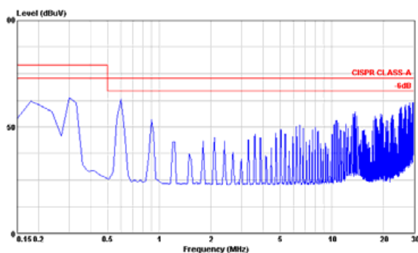
Conduction Emission of EN55022 Class A
