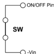
When TEP 150WI module is turned off at Low-level logic
