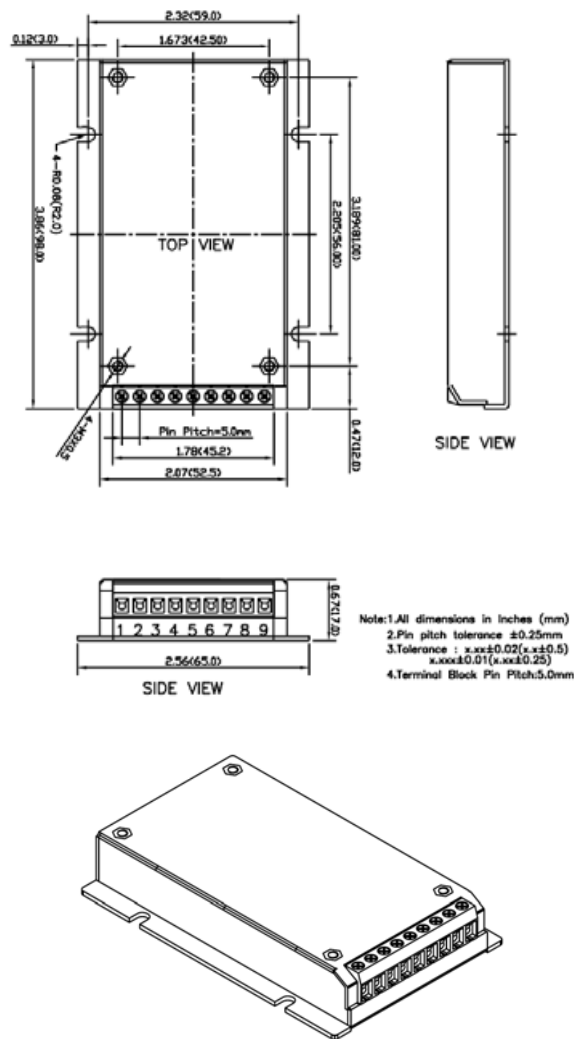
TEP 150WI DIMENSIONS
