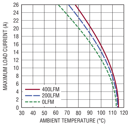
Figure 16. 5V to 1V Derating Curve, BGA Heat Sink
