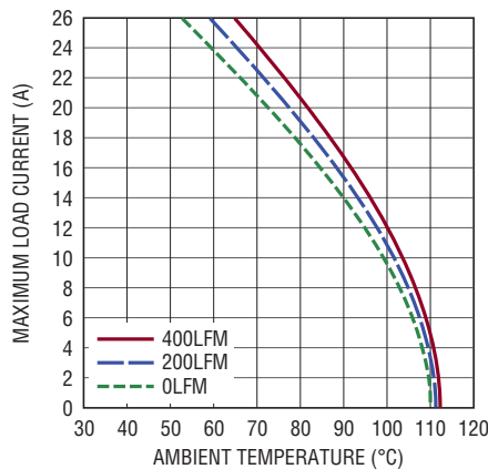
Figure 19. 5V to 1.8V Derating Curve, No Heat Sink
