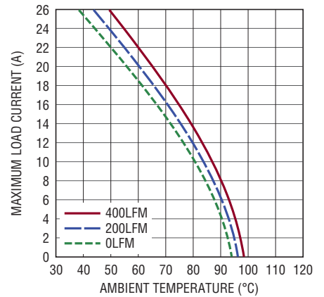
Figure 15. 24V to 1V Derating Curve, No Heat Sink
