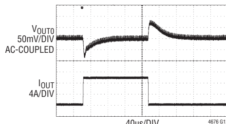
FIGURE 41 CIRCUIT AT 24\text{V}_{\text{IN}} , \text{C}_{\text{OUT}0} = 5 \times 100\mu\text{F} AND \text{VOUT}_0 COMMANDED TO 3.300\text{V} . 0\text{A} TO 10\text{A} LOAD STEP AT 10\text{A}/\mu\text{s}
