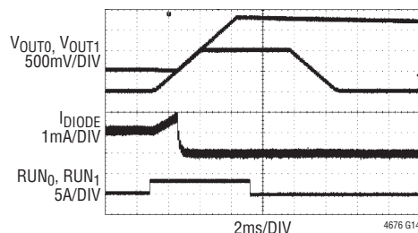
FIGURE 41 CIRCUIT AT 12\text{V}_{\text{IN}} , 77\text{m}\Omega LOAD ON \text{VOUT}_0 , 500\Omega ON \text{VOUT}_1 . \text{VOUT}_1 PRE-BIASED THROUGH A DIODE. \text{TON\_RISE}_0 = 3\text{ms} , \text{TON\_RISE}_1 = 5.297\text{ms} , \text{TOFF\_DELAY}_1 = 0\text{ms} , \text{TOFF\_DELAY}_0 = 2.43\text{ms} , \text{TOFF\_FALL}_1 = 5.328\text{ms} , \text{TOFF\_FALL}_0 = 3\text{ms} , \text{ON\_OFF\_CONFIG} = 0x1\text{F}
