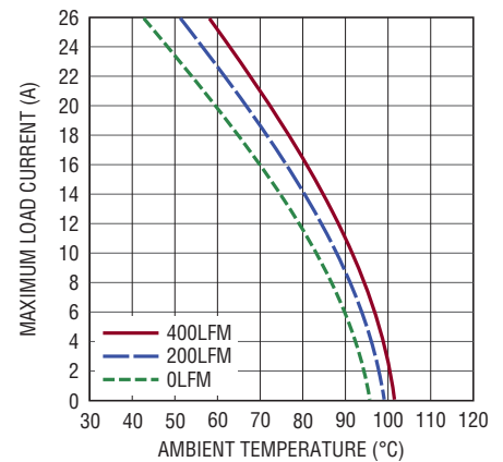
Figure 18. 24V to 1V Derating Curve, BGA Heat Sink
