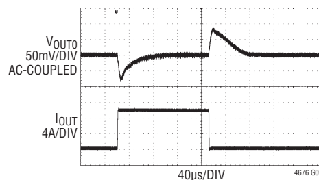
FIGURE 41 CIRCUIT AT 12\text{V}_{\text{IN}} , 0\text{A} TO 10\text{A} LOAD STEP AT 10\text{A}/\mu\text{s}
