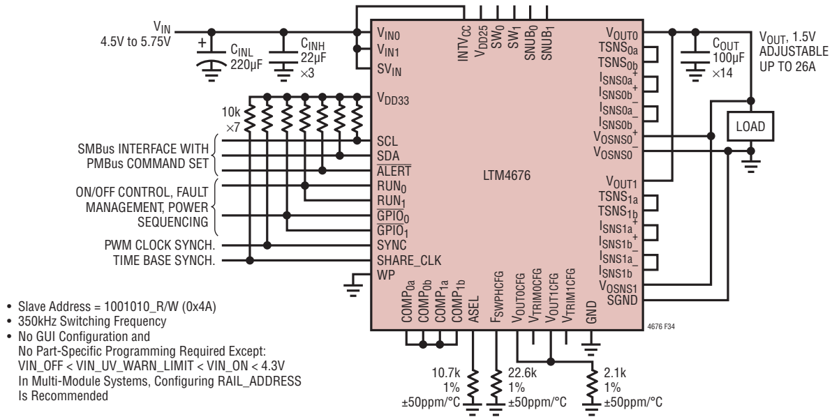
Figure 34. 26A, 1.5V Output DC/DC μModule Regulator with I 2 C/SMBus/PMBus Serial Interface
