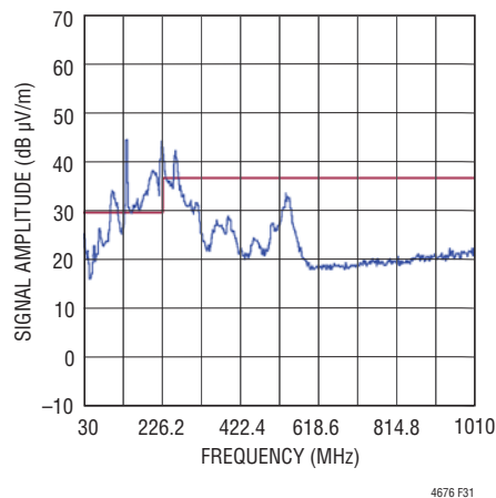
Figure 31. Radiated Emissions Scan of LTM4676 Producing 1V OUT at 26A, from 12V IN . DC1811 Hardware with Outputs Paralleled. No Snubbers Applied. f_{SW} = 350kHz. Measured in a 10m Chamber. Peak Detect Method
