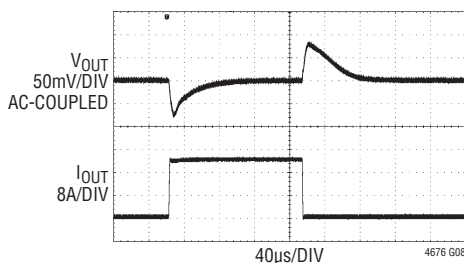
FIGURE 34 CIRCUIT AT 12\text{V}_{\text{IN}} , \text{INTV}_{\text{CC}} PIN OPEN CIRCUIT AND \text{VOUT\_COMMAND}_n SET TO 1.000\text{V} . 0\text{A} TO 20\text{A} LOAD STEP AT 20\text{A}/\mu\text{s}
