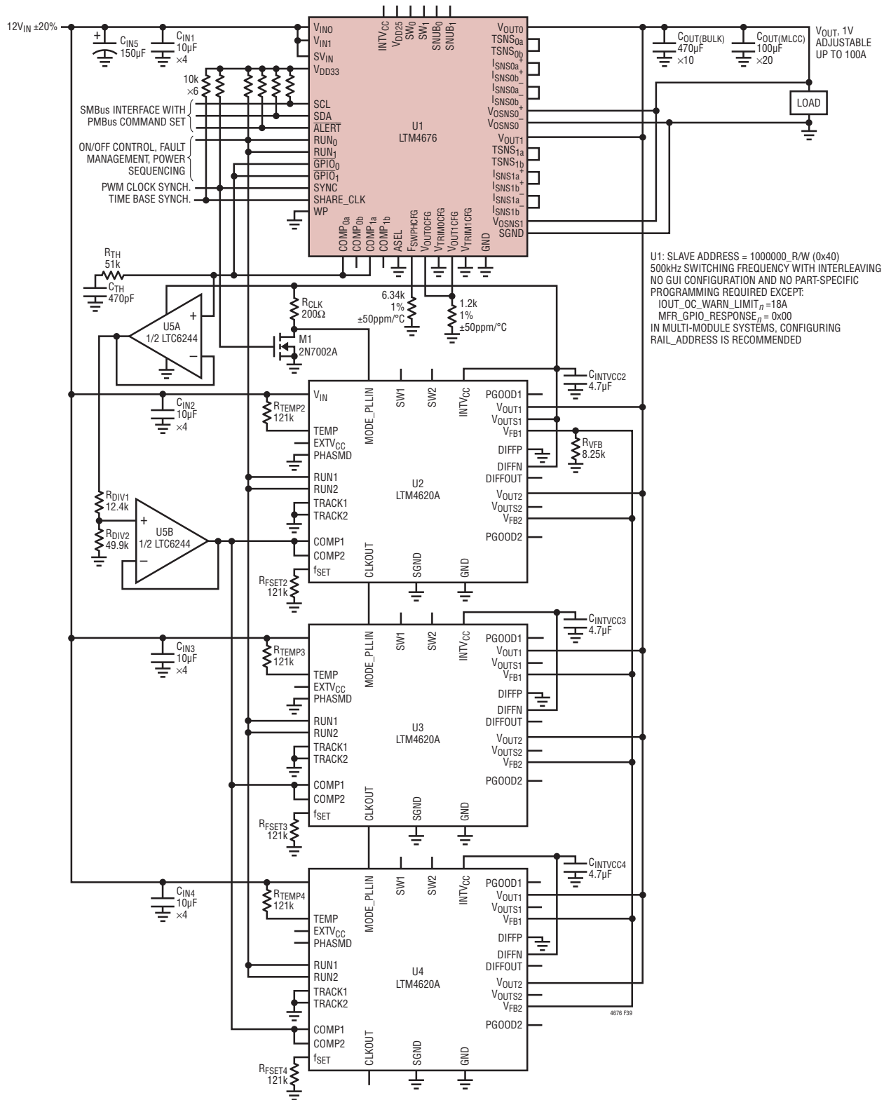
Figure 39. One LTM4676 Operating In Parallel with 3xLTM4620A (See Demo Board DC2106A-A) Producing 1V OUT at up to 100A. Power System Management Features Accessible Through LTM4676 Over 2-Wire I 2 C/SMBus/PMBus Serial Interface. See Figure 40
