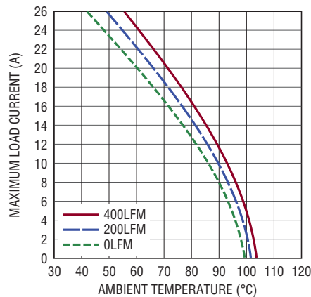
Figure 20. 12V to 1.8V Derating Curve, No Heat Sink
