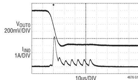
FIGURE 41 CIRCUIT AT 12\text{V}_{\text{IN}} , NO LOAD ON \text{VOUT}_0 PRIOR TO APPLICATION OF SHORT CIRCUIT
