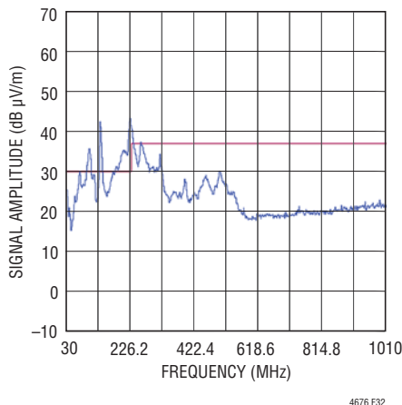
Figure 32. Radiated Emissions Scan of LTM4676 Producing 1V OUT at 26A, from 12V IN . DC1811 Hardware with Outputs Paralleled. 1Ω (1/4W rated) Snubber Resistors Applied from SNUB_n to GND. f_{SW} = 350kHz. Measured in a 10m Chamber. Peak Detect Method
