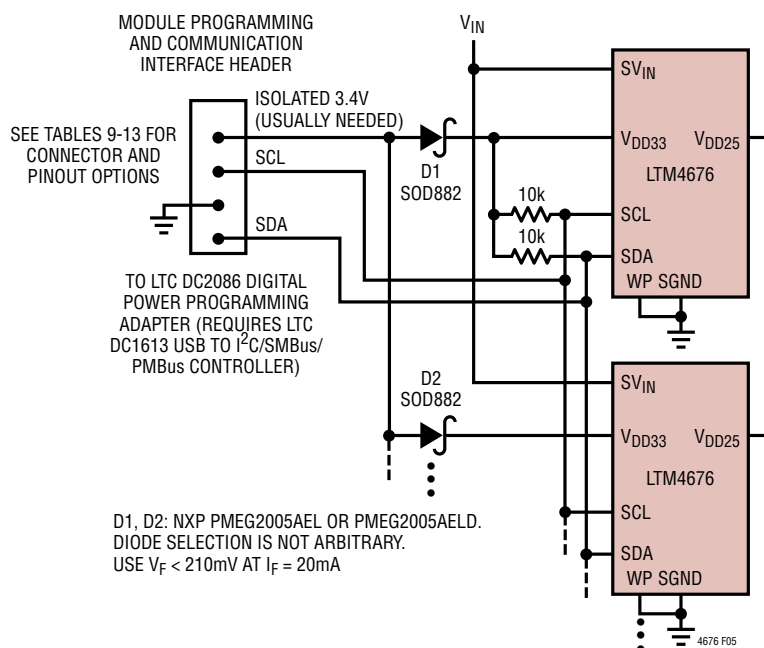
Figure 5. LTC Controller Connection Suitable for Programming NVM of Up to 16 LTM4676s When V IN Power is Absent, T A > 20°C and T J < 85°C
