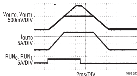
FIGURE 41 CIRCUIT AT 12\text{V}_{\text{IN}} , 77\text{m}\Omega LOAD ON \text{VOUT}_0 , NO LOAD ON \text{VOUT}_1 . \text{TON\_RISE}_0 = 3\text{ms} , \text{TON\_RISE}_1 = 5.297\text{ms} , \text{TOFF\_DELAY}_1 = 0\text{ms} , \text{TOFF\_DELAY}_0 = 2.43\text{ms} , \text{TOFF\_FALL}_1 = 5.328\text{ms} , \text{TOFF\_FALL}_0 = 3\text{ms} , \text{ON\_OFF\_CONFIG} = 0x1\text{E}
