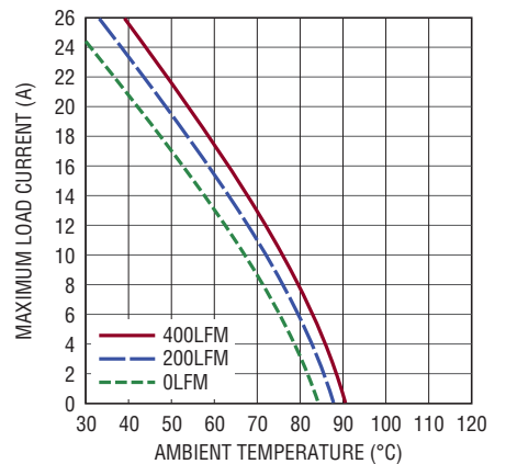
Figure 21. 24V to 1.8V Derating Curve, No Heat Sink
