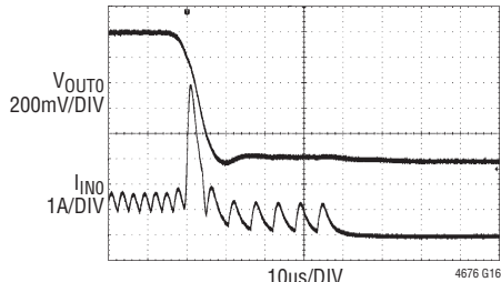
FIGURE 41 CIRCUIT AT 12\text{V}_{\text{IN}} , 77\text{m}\Omega LOAD ON V_{\text{OUT0}} PRIOR TO APPLICATION OF SHORT CIRCUIT
