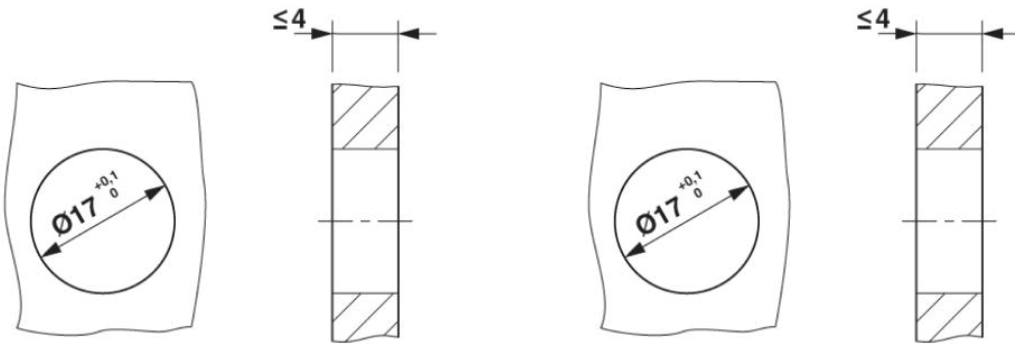
Panel cutout
