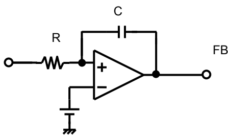
Fig.33 General integrator
