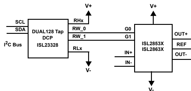
FIGURE 76. GAIN SWITCHING WITH ISL23328 DCP
