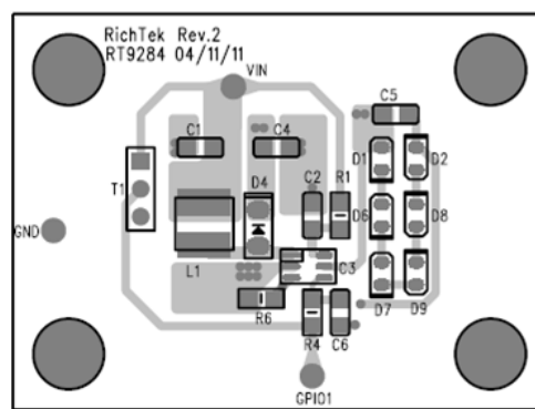
Figure 9. Top Layer
