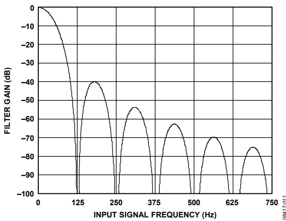
Figure 12. Filter Response
