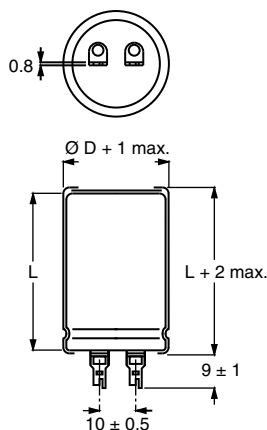
Fig. 10 - Solder-lug versions (SL): only available in 050 series
