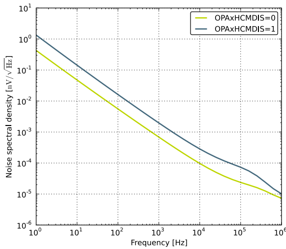
Figure 3.34. OPAMP Voltage Noise Spectral Density (Non-Unity Gain)
