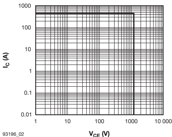
93196_02 V_{CE} (V) Fig. 2 - IGBT Reverse Bias SOA T_J = 150^\circ\text{C}, V_{GE} = 15\text{ V}
