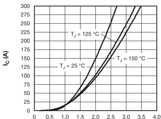
93196_03 V_{CE} (V) Fig. 3 - Typical IGBT Collector Current Characteristics V_{GE} = 15\text{ V}
