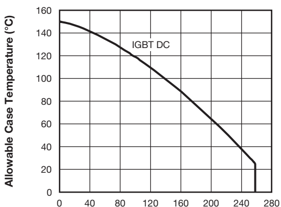
93196_01 I_C - Continuous Collector Current (A) Fig. 1 - Maximum DC IGBT Collector Current vs. Case Temperature
