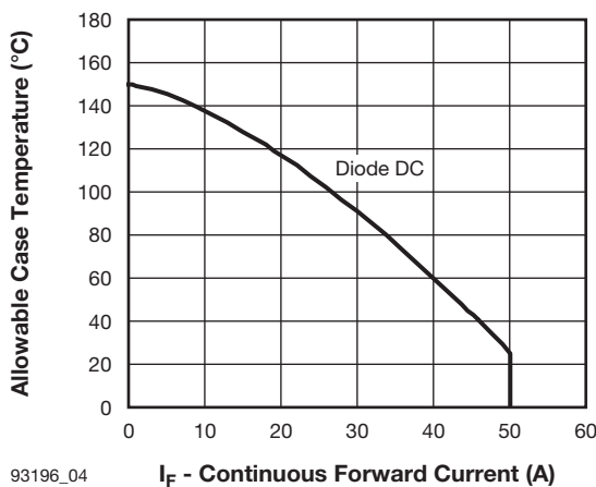
93196_04 I_F - Continuous Forward Current (A) Fig. 4 - Maximum DC Forward Current vs. Case Temperature
