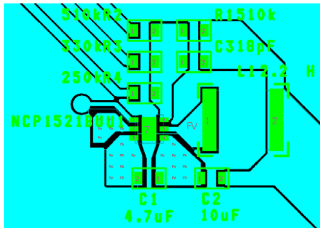
Figure 8. Part Layout in \mu DFN-6
