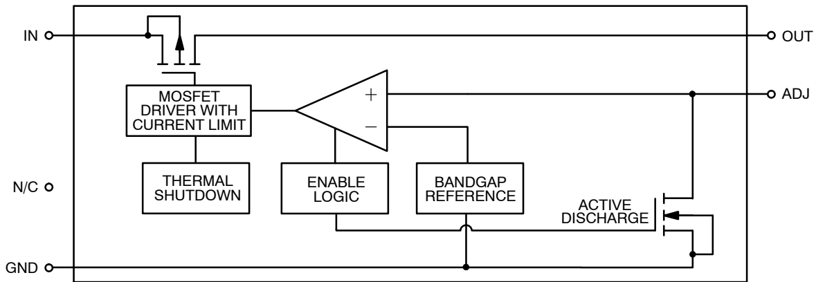
Figure 8. NCP690, NCV8690 Block Diagram (Adjustable Version)
