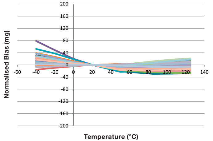
Figure 5.14: CAS214 (30g) Accelerometer X Bias variation with Temperature
