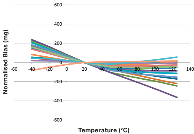
Figure 5.15: CAS215 (96g) Accelerometer X Bias variation with Temperature
