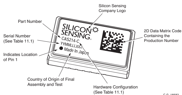
Figure 11.1 Part Marking
