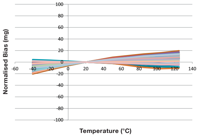
Figure 5.13 CAS213 (10g) Accelerometer X Bias variation with Temperature
