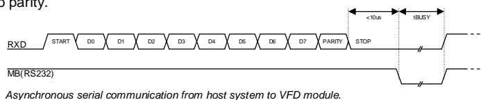
Asynchronous serial communication from host system to VFD module.
