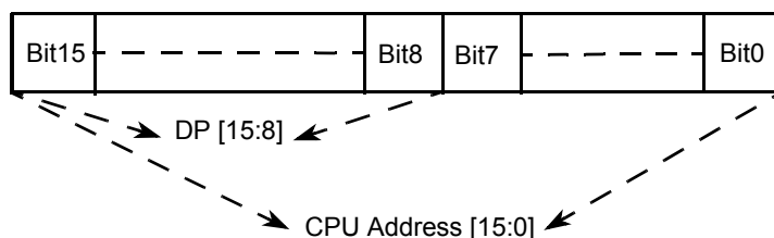
Figure 46. DIRECT Address Mapping
