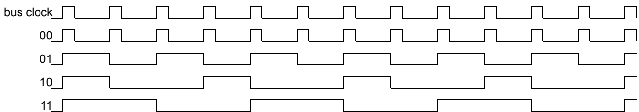
Figure 111. Interface Clock Waveforms for various D2DCLKDIV Encoding
