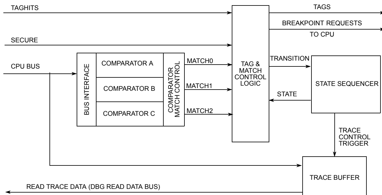
Figure 63. DBG Overview
