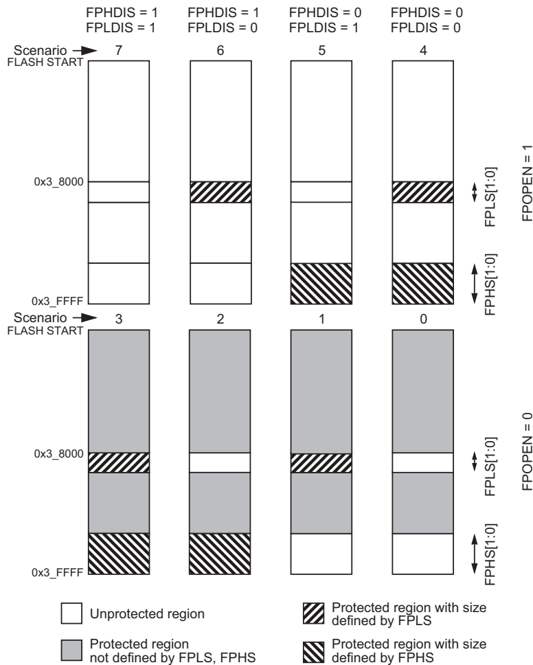
Figure 106. P-Flash Protection Scenarios
