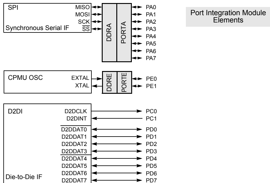
Figure 42. Block Diagram
