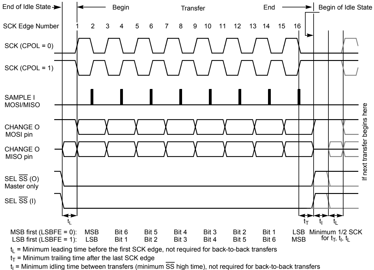
Figure 102. SPI Clock Format 1 (CPHA = 1), with 8-Bit Transfer Width Selected (XFRW = 0)
