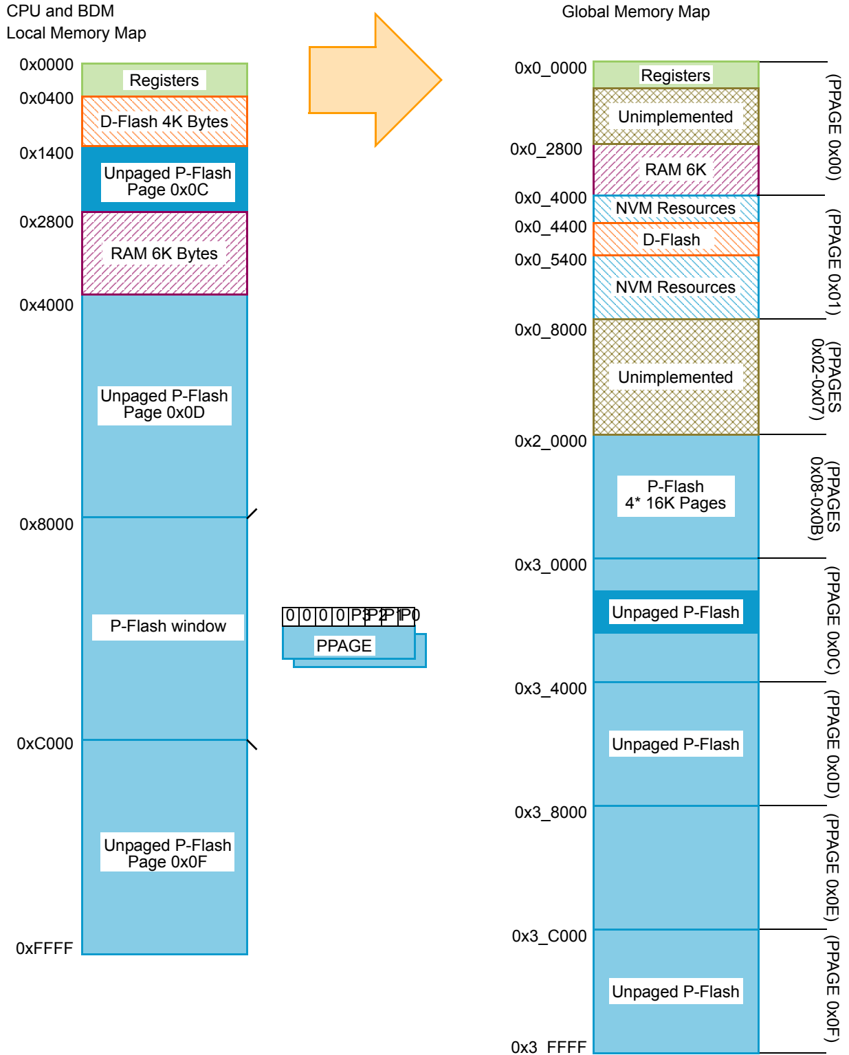
Figure 41. 9S121128 Global Memory Map
