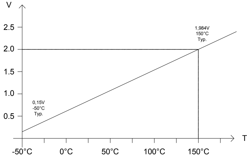
Figure 38. TSENSE - Graph
