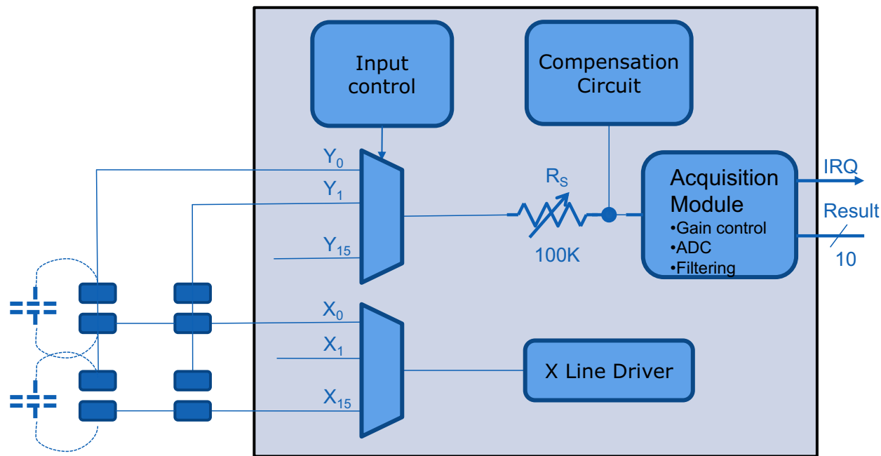
Figure 31-1. PTC Block Diagram Mutual-capacitance
