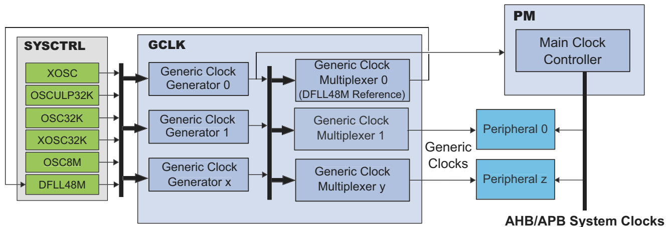
Figure 13-1. Clock distribution
