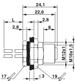
Dimensioned drawing
