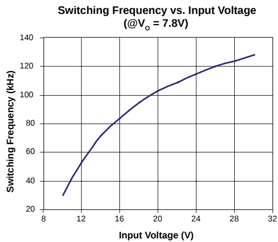
Fig. 9. Switching Frequency vs. Input Voltage Plot
