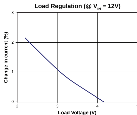
Fig. 4. Load Regulation of LED Current Plot
