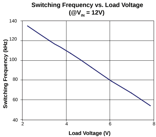
Fig. 10. Switching Frequency vs. Load Voltage Plot
