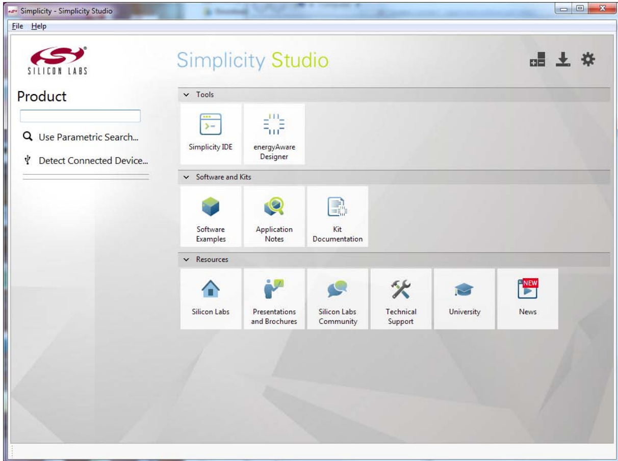
Figure 1. Simplicity Studio
