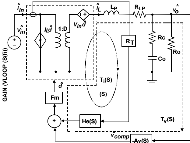
FIGURE 30. SMALL SIGNAL MODEL OF BUCK REGULATOR
