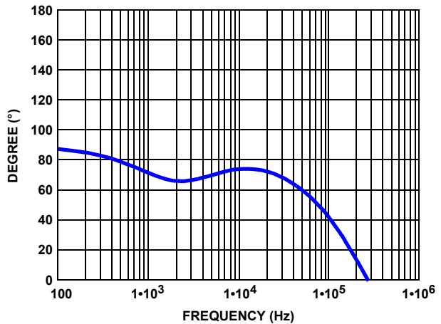
FIGURE 32. SIMULATED LOOP BODE PLOT
