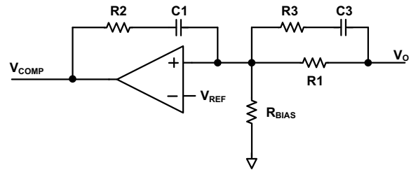
FIGURE 31. TYPE III COMPENSATOR
