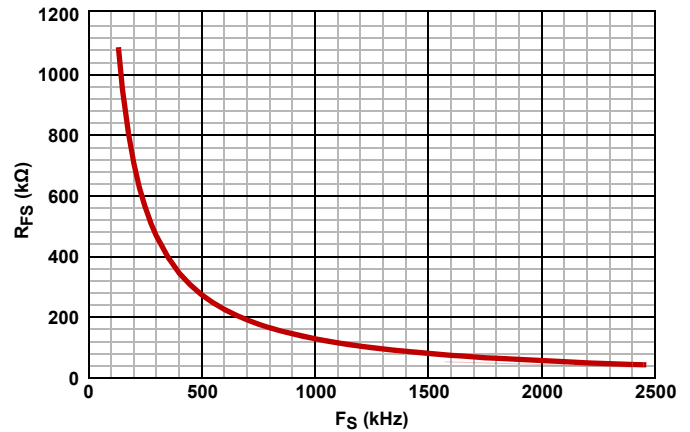
FIGURE 28. R FS vs FREQUENCY
