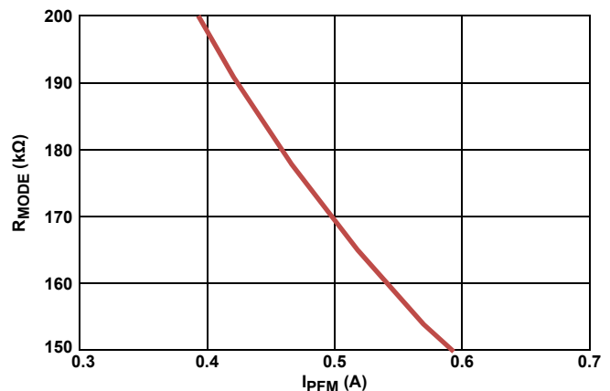
FIGURE 26. R MODE vs I PFM
