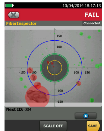
FiberInspector probe
