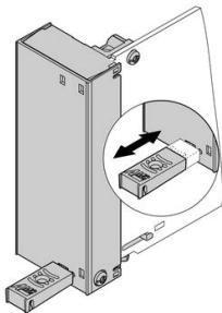
Pull-handle mechanism
