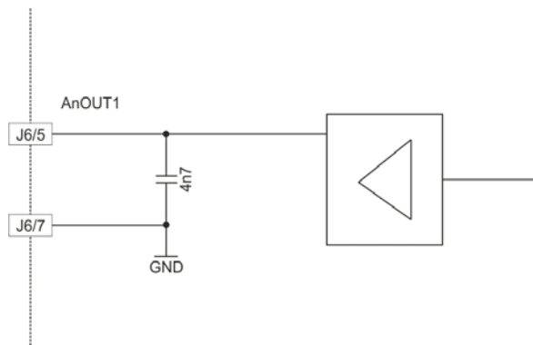
Figure 3-17 AnOUT1 Circuit (analogously valid also for AnOUT2)
