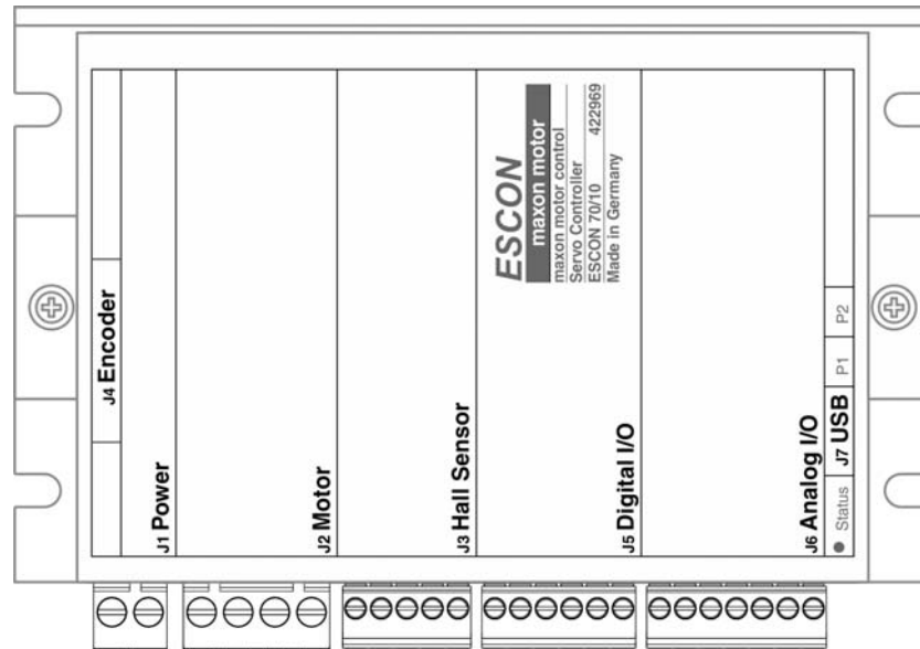
Figure 4-21 Interfaces – Designations and Location
