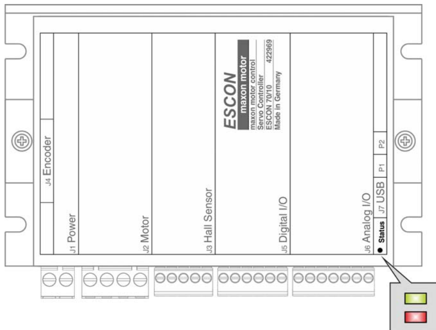
Figure 3-20 LEDs – Location
