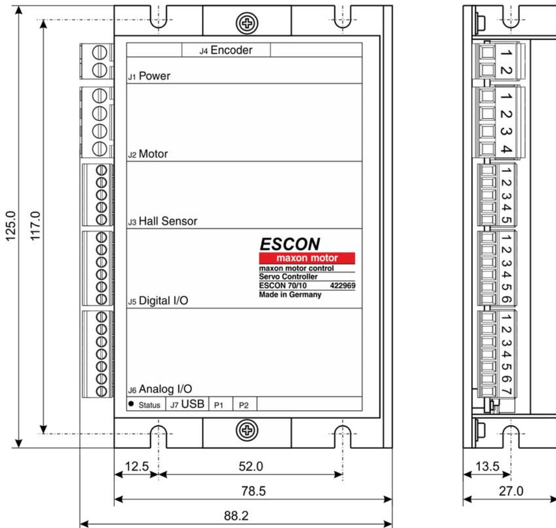
Figure 2-1 Dimensional Drawing [mm]
