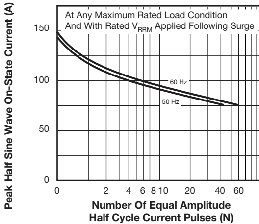
Fig. 7 - Maximum Non-Repertitive Surge Current vs. Number of Current Pulses, 2N681 Series
